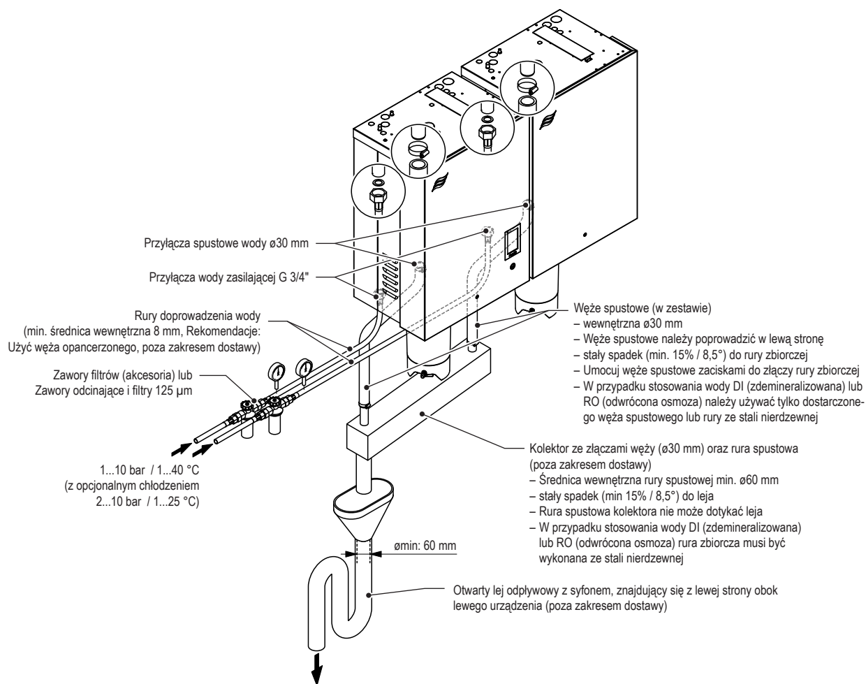
Rys. 24: Overview water installation for double units Medium ("M ")
