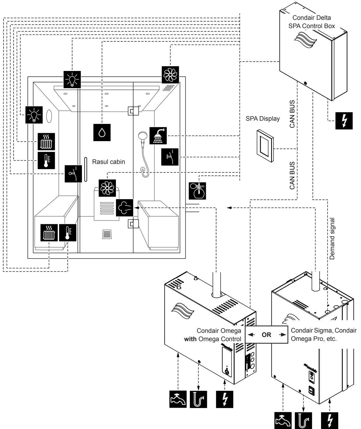
Fig. 7: Condair Delta SPA Control Box with equipment for Rasul application
